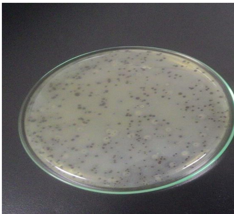
Figura 18 – Staphylococcus aureus
