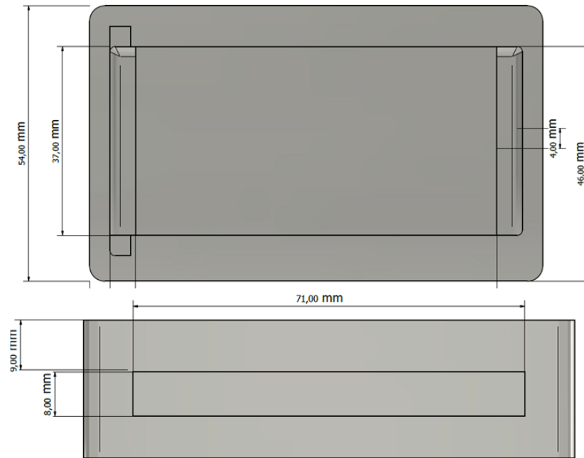
Figura 33 – MobileSPR Case 2.0 - Base.
