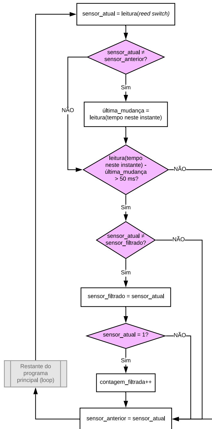
Figura 21: Fluxograma do filtro digital ( debounce ).
